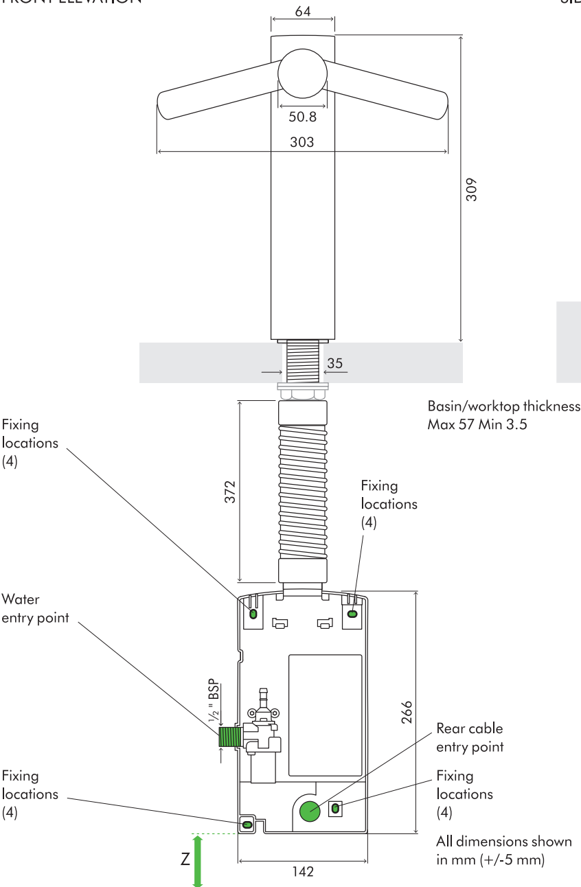
FRONT ELEVATION
